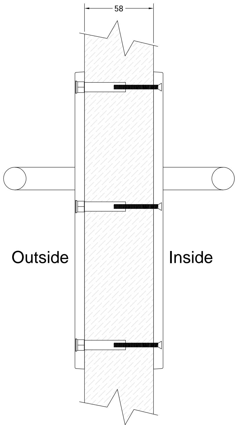
Assembled View
