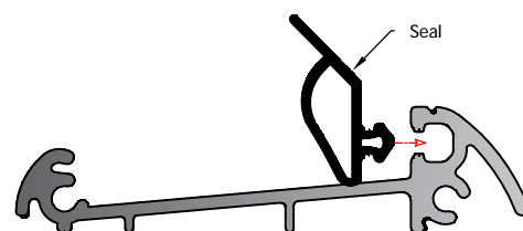
Exploded View
