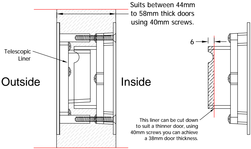
Section C-C
