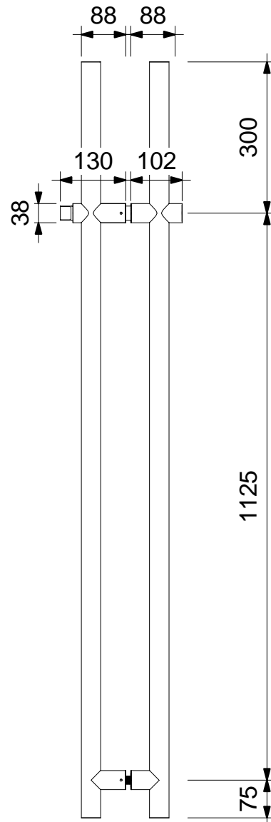
③ Front View 1 : 7
