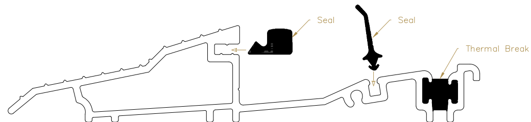
Exploded View
