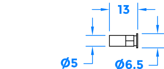
2 x Bolt Receiver Sleeve
