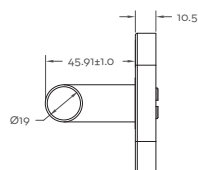
Top Profile
