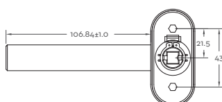
Rear Profile
