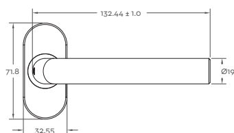
Rear Profile
