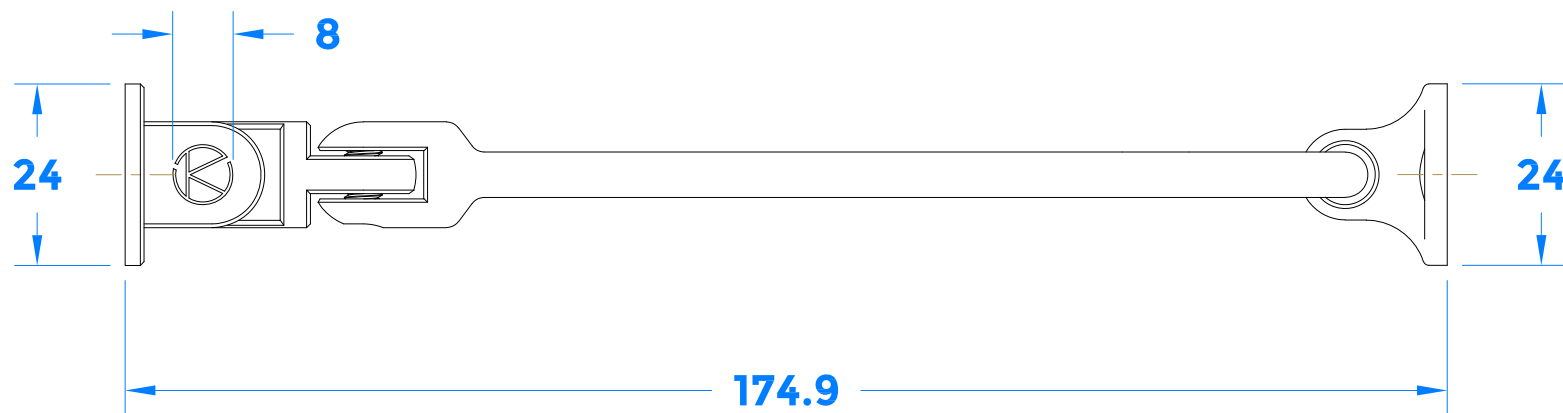
TOP VIEW
