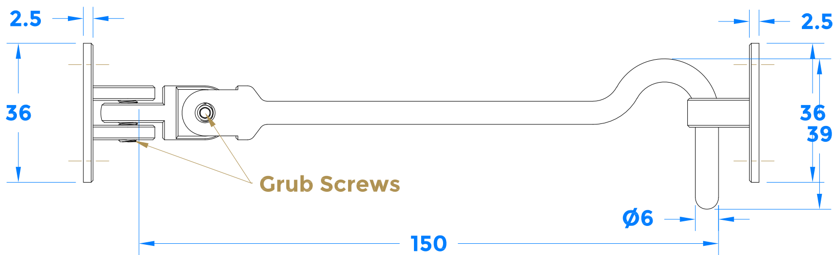
SIDE VIEW
