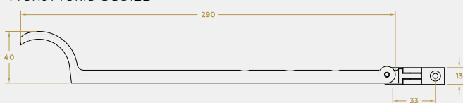
Front Profile CC812B
