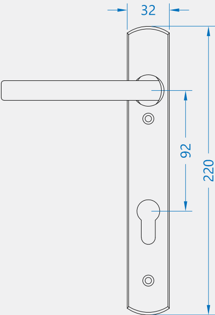
Front Profile
