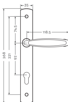
Front Profile
