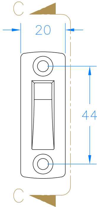
Mortice Plate
