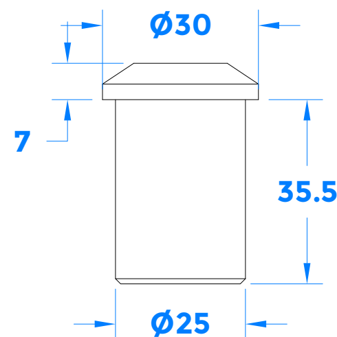
Sprung Loaded Floor Keep
