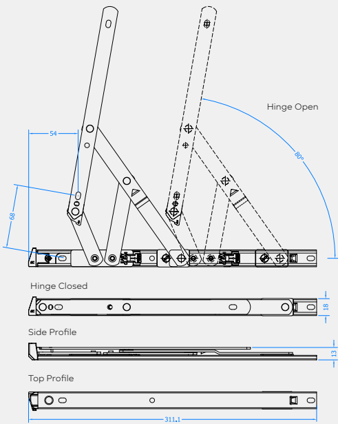
Hinge Project Out Dimension
