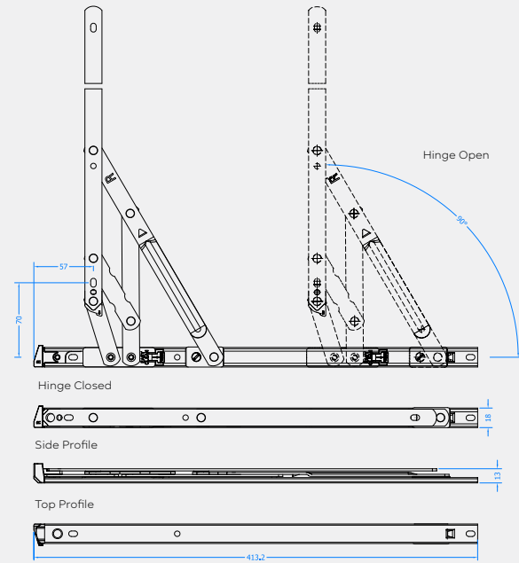
Hinge Project Out Dimension
