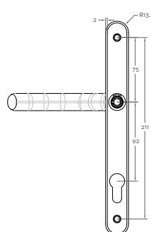
Rear Profile
