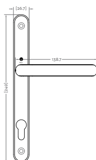
Front Profile
