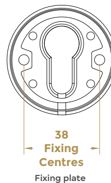
Front Profile
