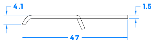
Section B-B
