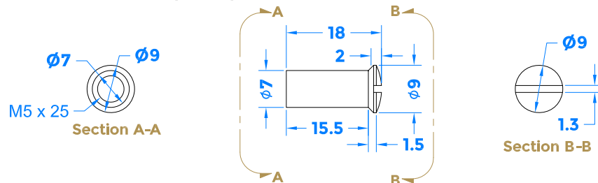
Hollow Bolt Receiver (FX-390)
