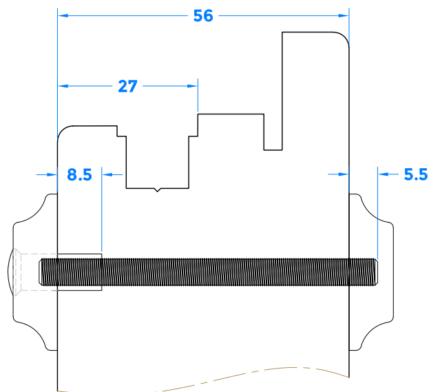
Assembled View
