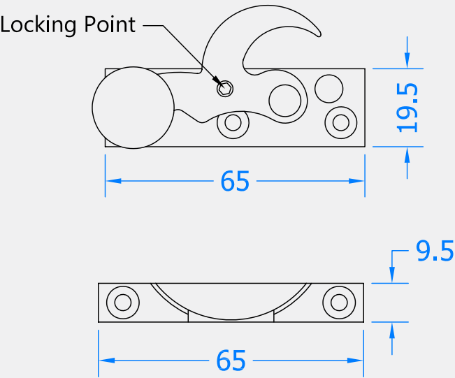
Top Profile
