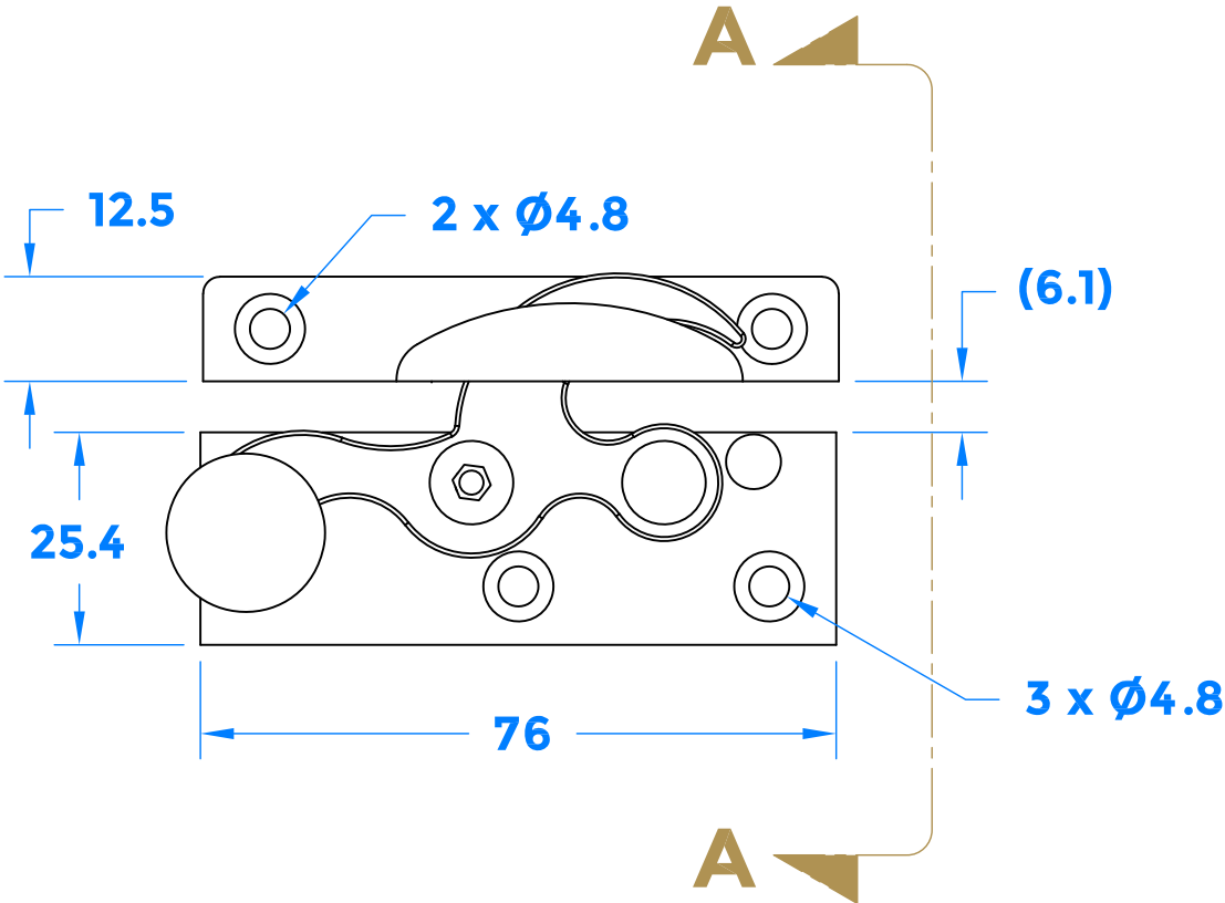
Closed View
