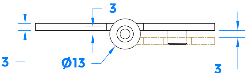
Section A-A Top View
