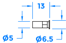
2 x Bolt Receiver Sleeve
