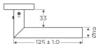
Top Profile
