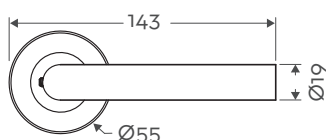
Front Profile
