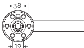
Rear Profile
