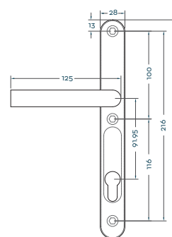
Rear Profile
