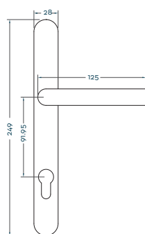
Front Profile
