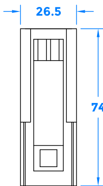
Spring Cassette
