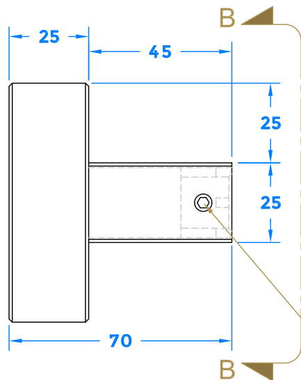
Side View Section A-A
