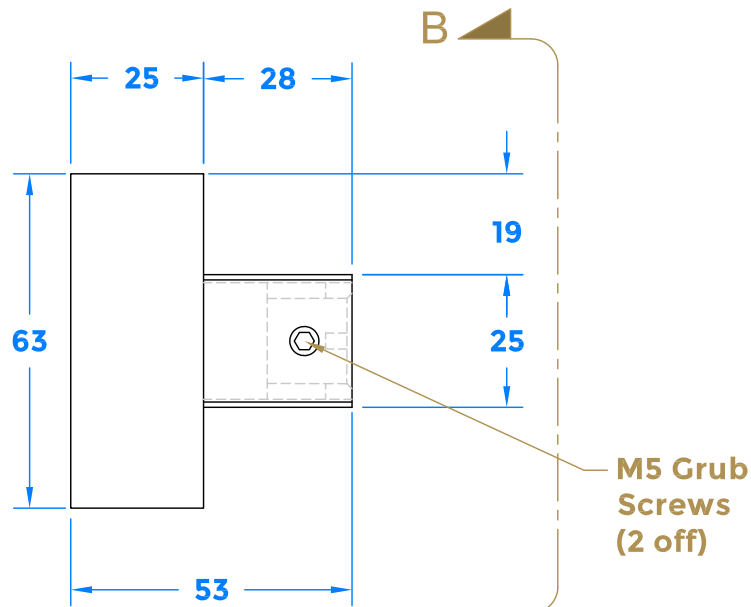
Side View Section A-A
