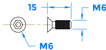
Fixing Bolt
