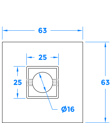
Rear View Section B-B
