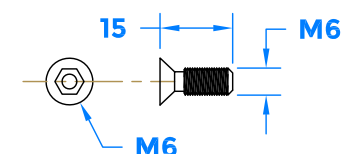
Fixing Bolt
