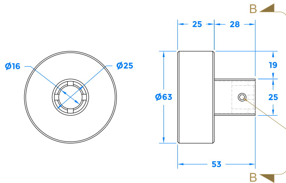
Rear View Section B-B
