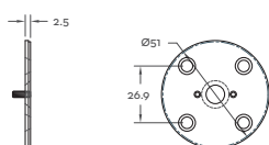
Fixing Plate
