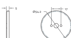
Cover Plate
