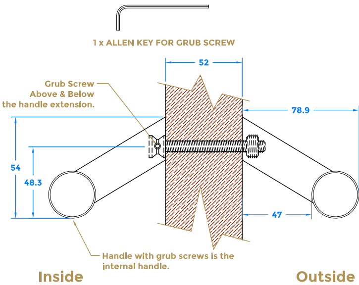
Assembled View (Back to Back)
