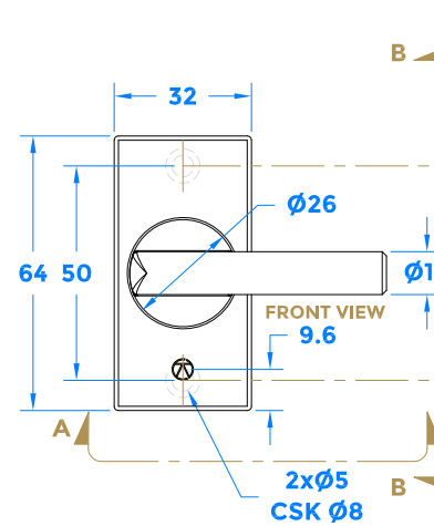
Backplate
