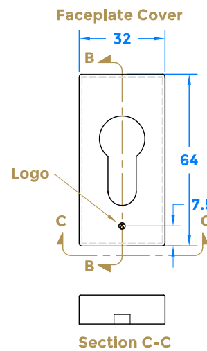
Section C-C
