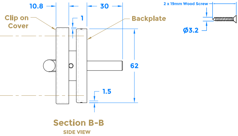
Faceplate Cover
