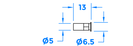
2 x Bolt Receiver Sleeve
