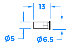
2 x Bolt Receiver Sleeve
