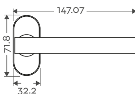
Front Profile
