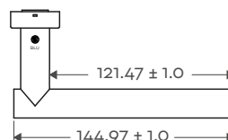
Top Profile
