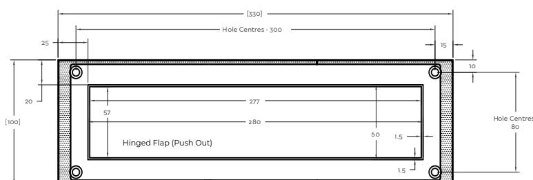
LP430-PSS Polished Stainless Steel
