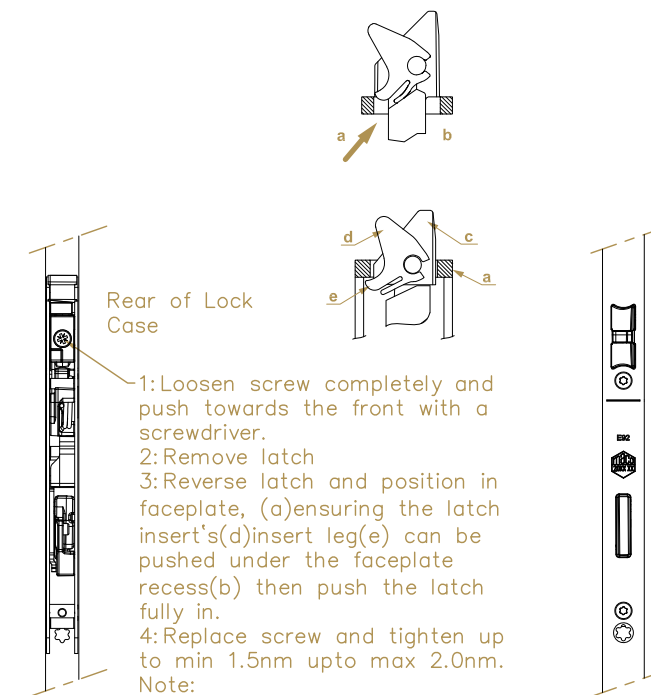
Detail A Latch Release
