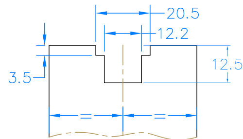
SECTION B-B EURO GROOVE
