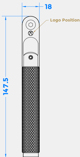
Front Profile
