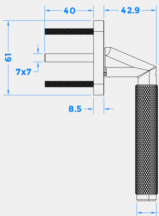
Side Profile
