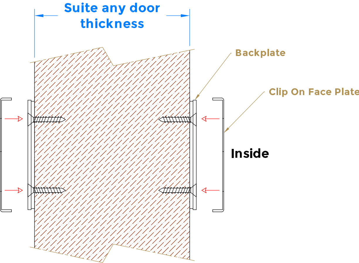
Assembled View
