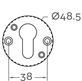
Fixing Plate
