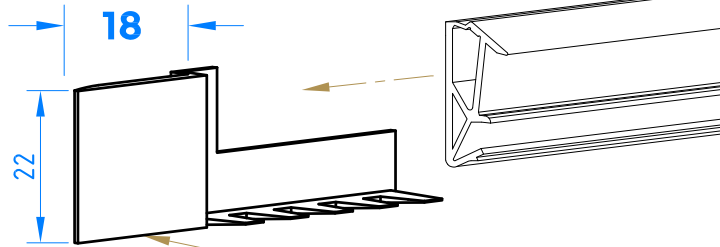
SP-VESU22 For a 15mm Rebate
