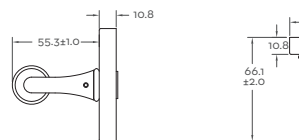
Side Profile
