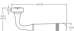
Top Profile
