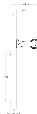
Side Profile
