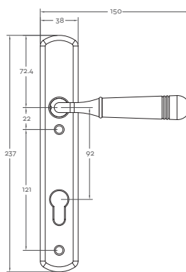
Front Profile
