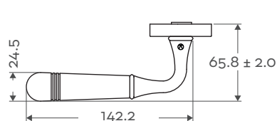
Top Profile
