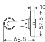
Side Profile
