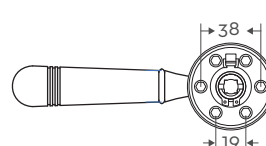
Rear Profile
