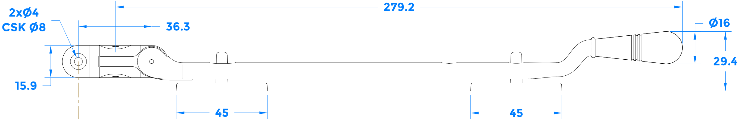
Side View
