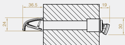
Section through slot
