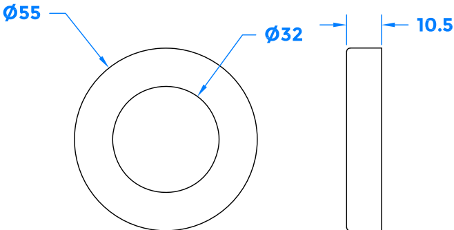
Cover Plate
