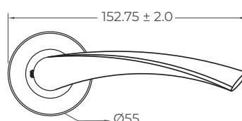
Front Profile
