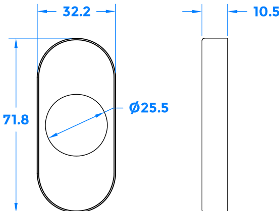
Cover Plate
