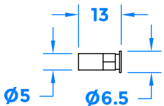
2 x Bolt Receiver Sleeve
