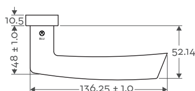
Top Profile
