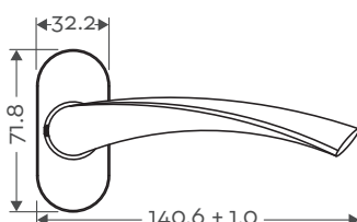
Front Profile
