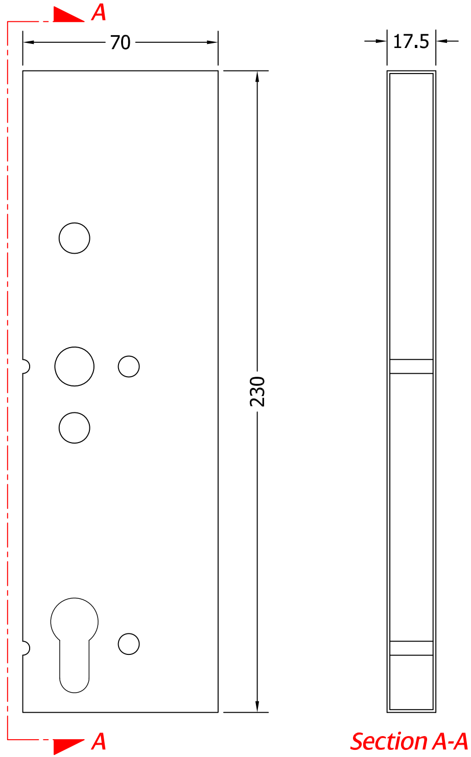
Centre Gearbox Cover
