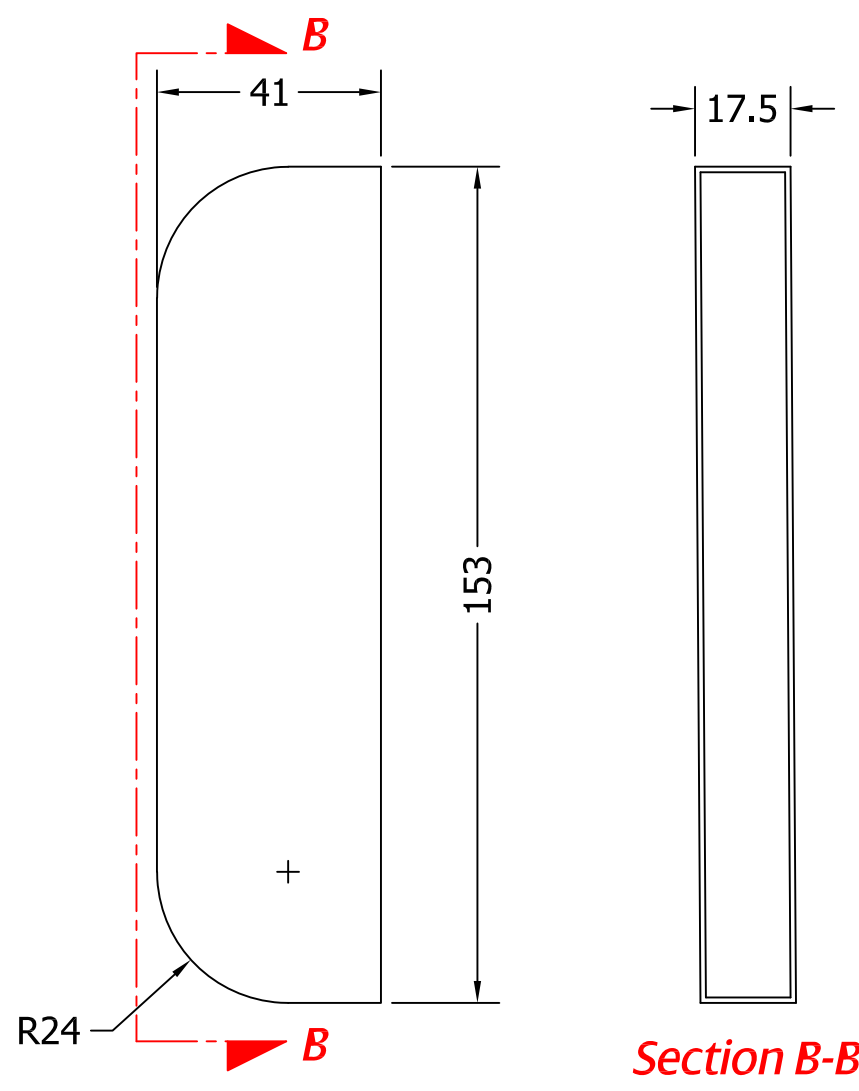
Top/Bottom Gearbox Cover
